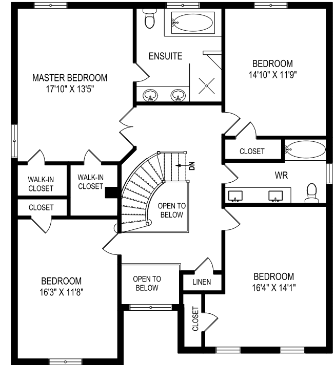
SECOND FLOOR 1506 SQUARE FEET AREA INCLUDES 55 SQUARE FEET OPEN TO BELOW SPACE
